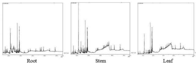
Figure 1: GC-MS chromatogram of the methanol extract of various parts of Ceropegia bulbosa Roxb. var. lushii (Grah.) Hook.f
