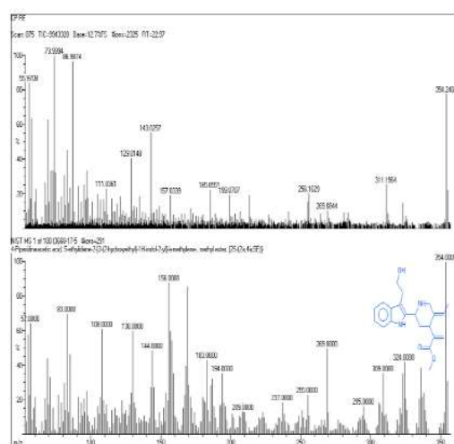
Figure 5: Mass spectrum of 4-Piperidineacetic acid, 1-acetyl-5- ethyl-2- (3,2-hydroxyethyl)-1H-indol-2-yl)-a-methyl methyl ester (RT: 22.97) from extracellular protein fraction of Bacillus subtilis SK09
