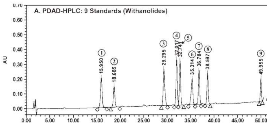
Figure 1: Test set of Withanolides by HPLC
