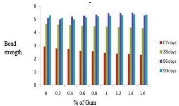
Figure 4: Bond Strength of concrete using different gum percentages
