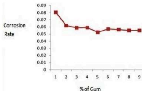
Figure 5: Corrosion rates from weight loss method
