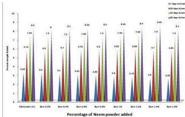
Figure 3: Flexural strength of concrete beams
