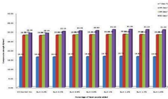
Figure 1: Compressive strength of concrete cubes
