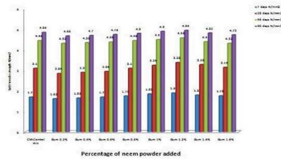
Figure 2: Split tensile strength of concrete cylinders
