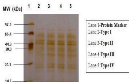
Figure 1: SDS PAGE depicting protein profile of Type I, Type II, Type III and Type IV casted with 10 % Agarose Gel Electrophoresis
