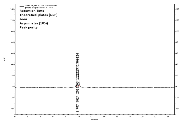
Figure 3: Chromatogram of degraded sample
