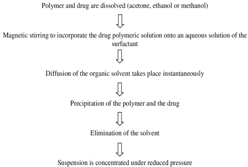
Figure 3: Schematic flow of Nanoprecipitation method 81
