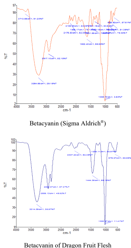
Figure 1: The FTIR spectra of betacyanin at wave numbers 600-4000 cm -1
