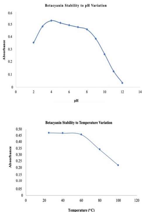
Figure 2: Betacyanin Stability to pH and Temperature
