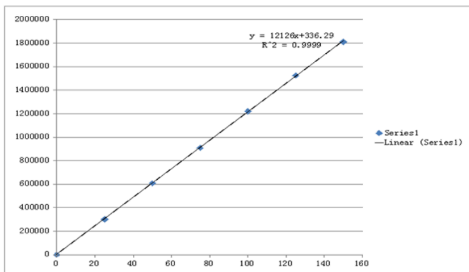
Figure 3: Calibration curve of Paracetamol
