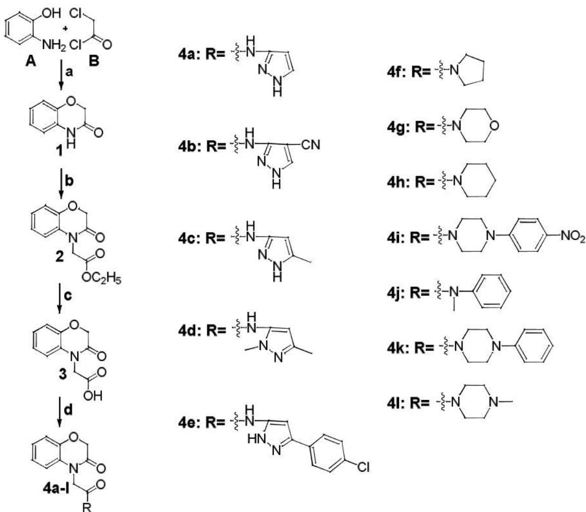
Scheme 1: a) TEBA, \text{CHCl}_3 , \text{NaHCO}_3 , 0-5°C for 1 h and 55°C for 12 h, b) \text{K}_2\text{CO}_3 in acetonitrile for 30 mins, TBAI for 12 h, c) LiOH, THF for 12 h, d) HOBT, EDC. HCl, DCM for 30 mins, trimethylamine for 12 h.
