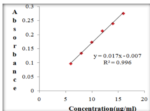
Figure 5: Calibration curve for TENE at 233 nm
