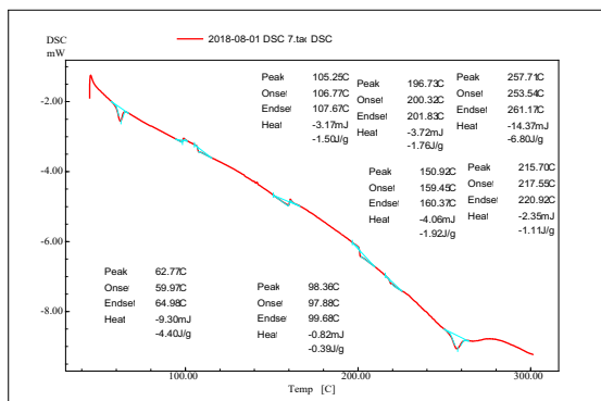
DSC thermogram of Pure drug + Epichlorohydrin - Beta cyclodextrin
