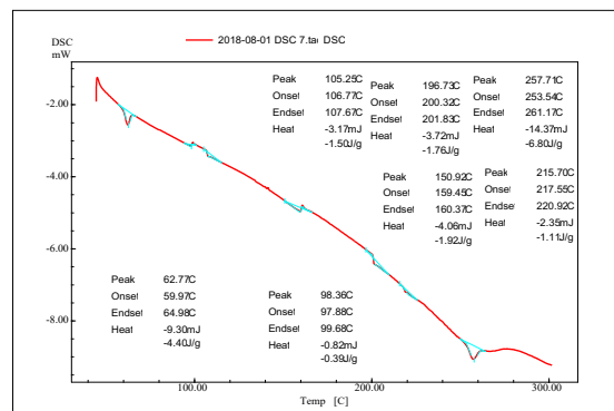
DSC thermogram of Pure drug + sulfobutylether cyclodextrin
