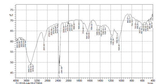
FT-IR Spectrum of Pure drug + Sulfobutyl ether cyclodextrin (SBECD)
