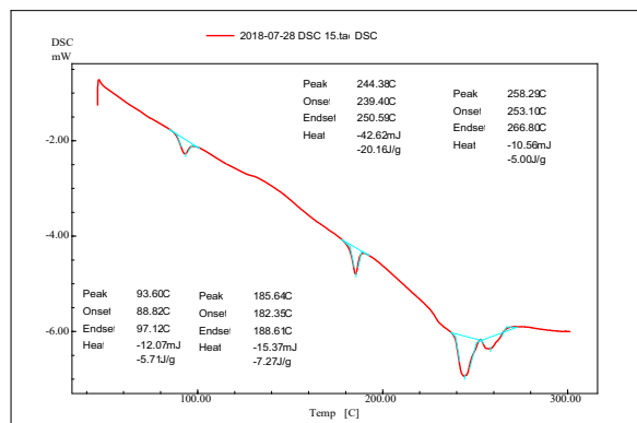
DSC thermogram of of Pure drug + Beta cyclodextrin
