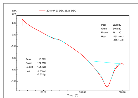
DSC thermogram of Pure drug
