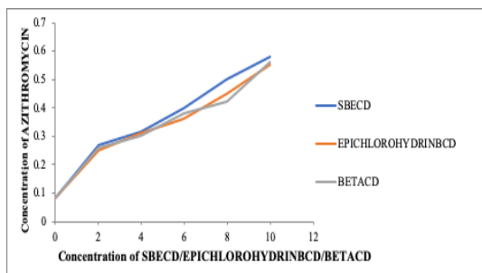
Figure 5: Phase solubility studies
