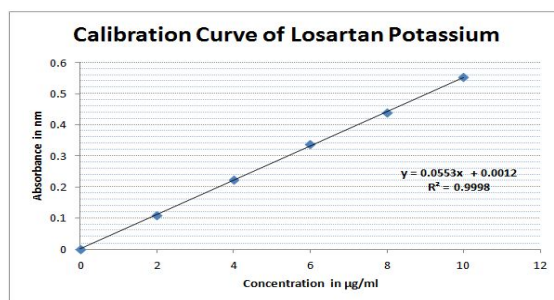
Figure 3: Calibration Curve of Losartan potassium
