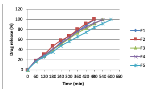
Figure 9: In-vitro Release graph
