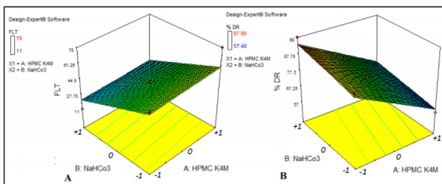
Figure 2: 3D diagram A- Effect of X1 and X2 on Y1. B- Effect of X1 and X2 on Y2
