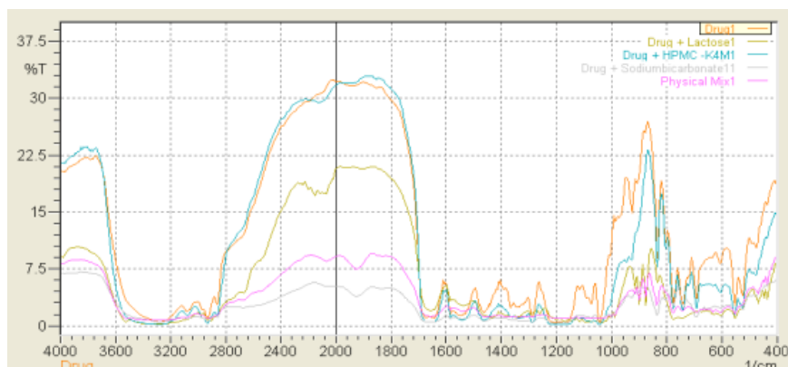
Figure 1: Overlay spectra of Nevirapine, HPMC K4M, lactose and physical mixture
