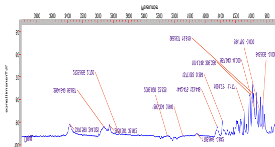
Figure 1: FTIR spectra of DHA
