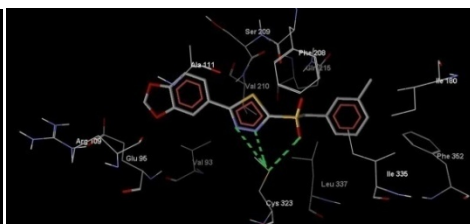
Figure 2: Docking pose of (SP-150)
