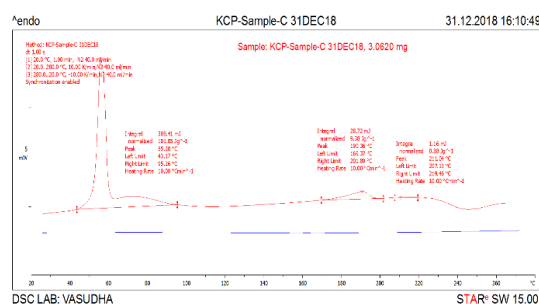
Figure 4: DSC of pure Docetaxel drug and Pluronic F68
