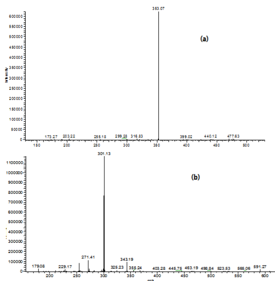
Figure S4: MS/MS fragmentation of Isochlorogenic acid b or c [M - H]^- (m/z) at 515.09; (b) MS2 of Rutin at [M - H]^- (m/z) at 609.26
