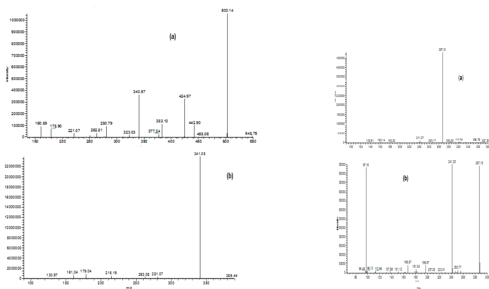
Figure S2: Negative ion ESI-MS/MS spectra of trisaccharide dihydrate at (a) MS2 of [M - H]^- ( m/z ) at 539.19; (b) MS3 fragmentation of main daughter ion disaccharide dihydrate at [M - H]^- ( m/z ) at 377.09
