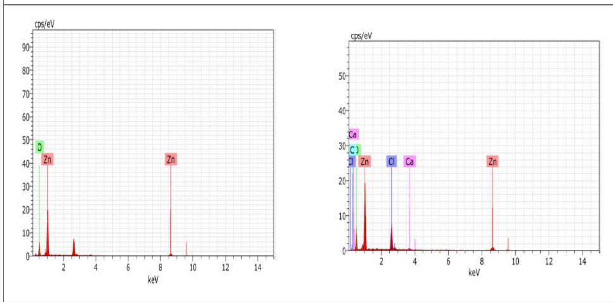
Figure 3: EDAX of Zinc Oxide Nanoparticles
