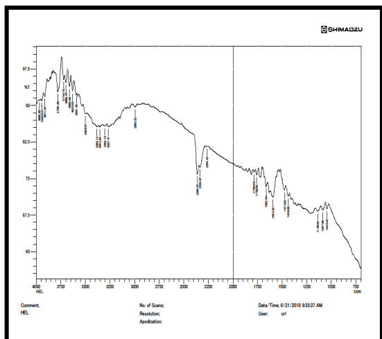
Figure 3: FTIR absorption spectrum of the hydroethanolic extract of leaf
