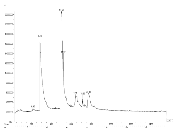
Figure 2: GC MS analysis of hydroethanolic extract of bark of A.saman
