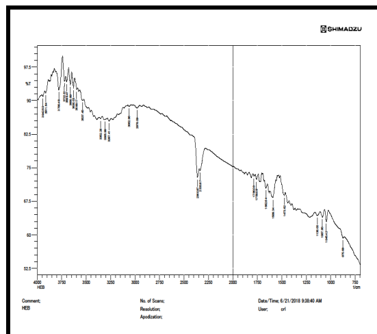
Figure 4: FTIR absorption spectrum of the hydroethanolic extract of bark
