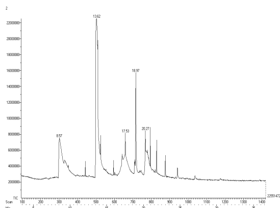
Figure 1: GC MS analysis of hydroethanolic extract of leaf of A.saman
