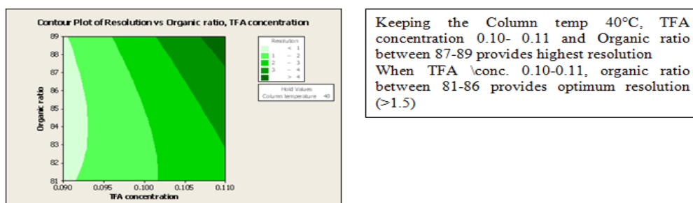
Figure 5: Contour plot for interaction between Organic ratio and TFA concentration
