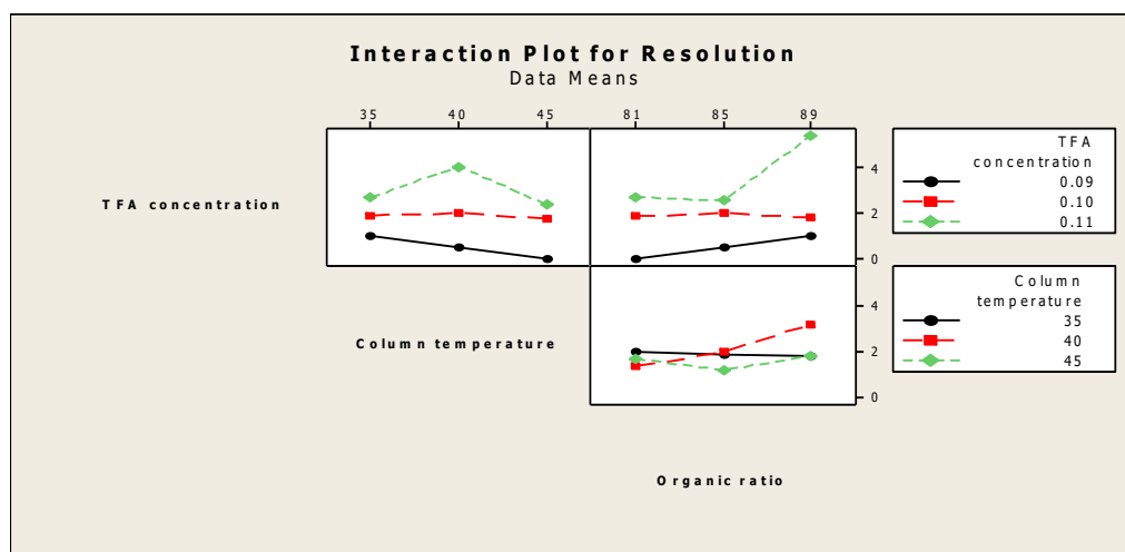
Figure 3: Interaction Plot for resolution of three CQAs
