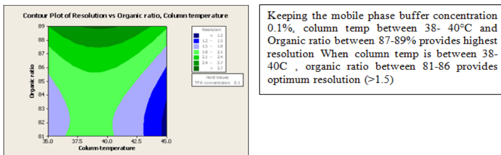
Figure 4: Contour plot for interaction between Organic ratio and Column Temperature
