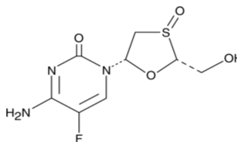
S-Oxide
