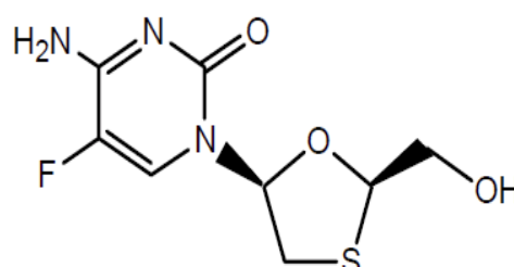
Emtricitabine (FTC)
