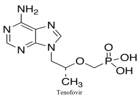
Figure 2: Structure of Tenofovir and S-Oxide impurities
