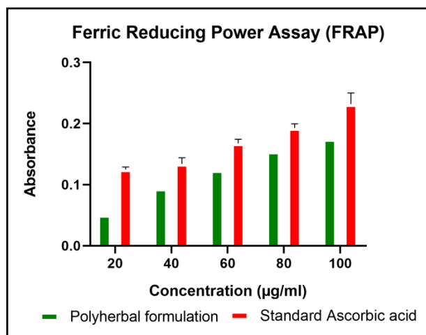
Figure 6: Ferric Reducing Power Assay (Absorbance)
