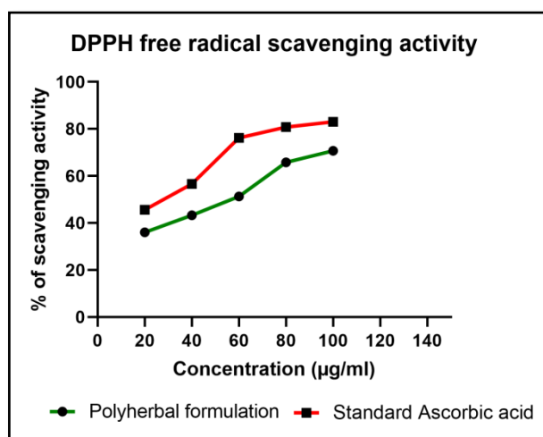
Figure 1: DPPH free radical scavenging activity
