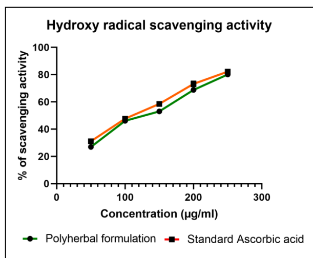
Figure 4: Hydroxy radical scavenging activity
