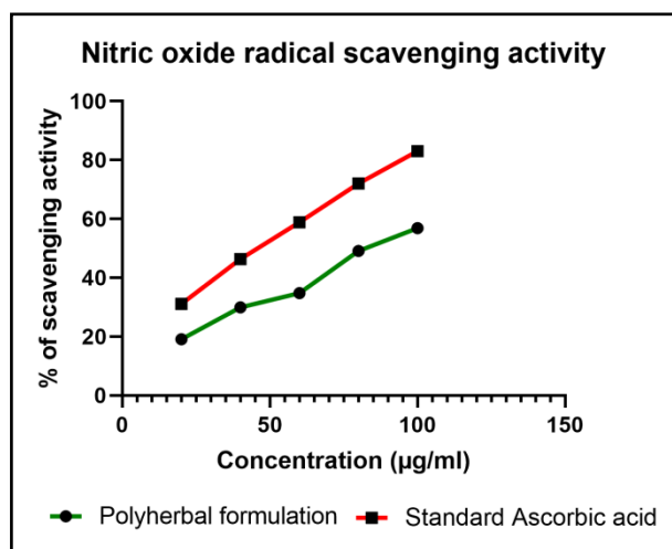
Figure 2: Nitric oxide free radical scavenging activity
