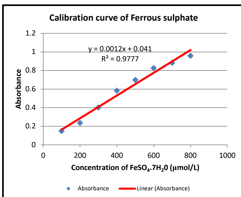
Figure 7: Calibration curve of Ferrous sulphate
