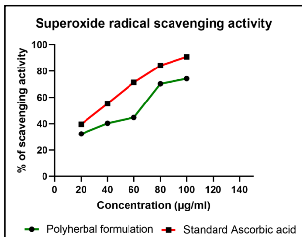
Figure 3: Superoxide radical scavenging activity
