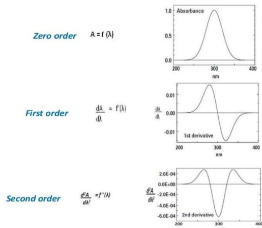
Figure 2: Zero, First & Second order derivative spectrum
