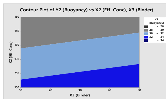
Fig 5: Contour Plot of Y2 (Buoyancy) Vs X2 (Effervescent Concentration) & X3 (Binder)
