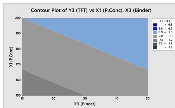
Fig 6: Contour Plot of Y3 (Total Floating Time) Vs X1 (Polymer Concentration) & X3 (Binder)
