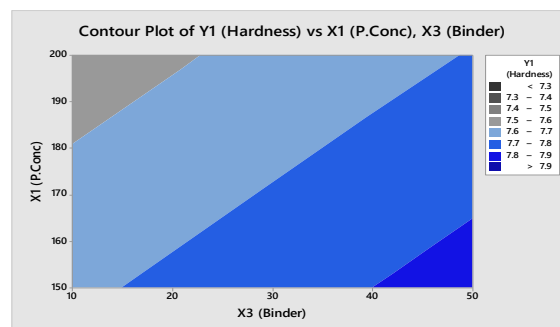
Fig 4: Contour Plot of Y1 (Hardness) Vs X1 (Polymer Concentration) & X3 (Binder)
