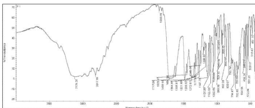
Fig. 1: FTIR of pure Domperidone
