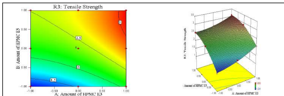
Figure 8: Contour plot and 3D Surface Plot of tensile strength (N/cm 2 ) against amount of HPMC E3 (%w/v) and amount of HPMC E5 (%w/v)
