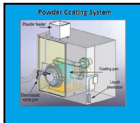
Figure 5. Electrostatic Powder Coating System 7
