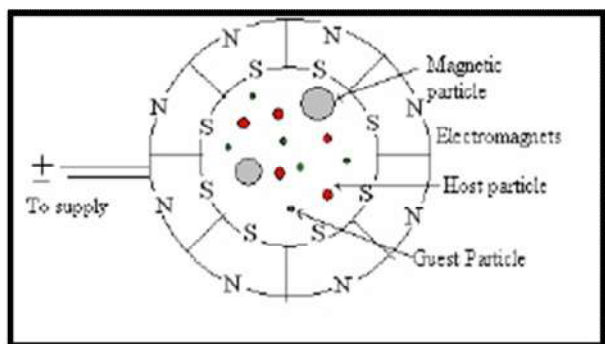
Figure 7:- Schematic diagram of MAIC
