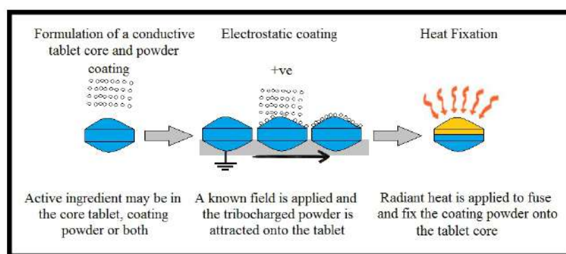
Figure 6: Schematic diagram of electrostatic dry coating.
