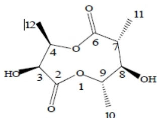
Fig 4. Lactone
