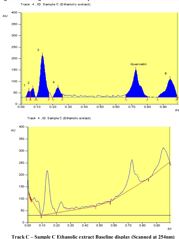
Figure. 6: Densitogram and Baseline for phenol of ethanolic extract of Barleria cristata
