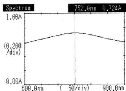
Figure 1: Spectra of ceftazidime with FC reagent in presence of sodium carbonate in distilled water showing maximum absorbance at 752 nm
