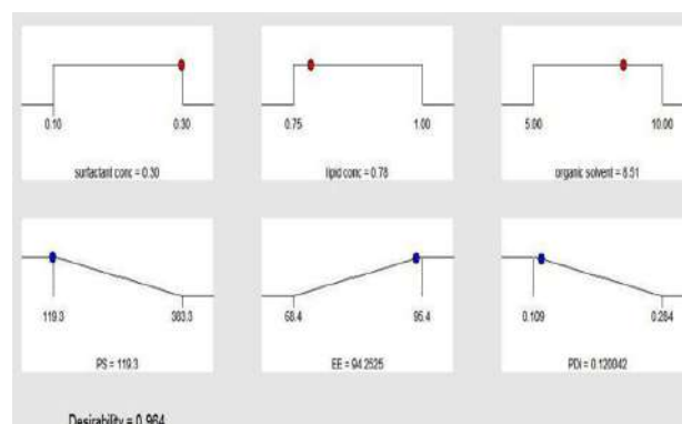
Figure 8: Predicted levels of various responses based on numerical optimization of desirability approach
