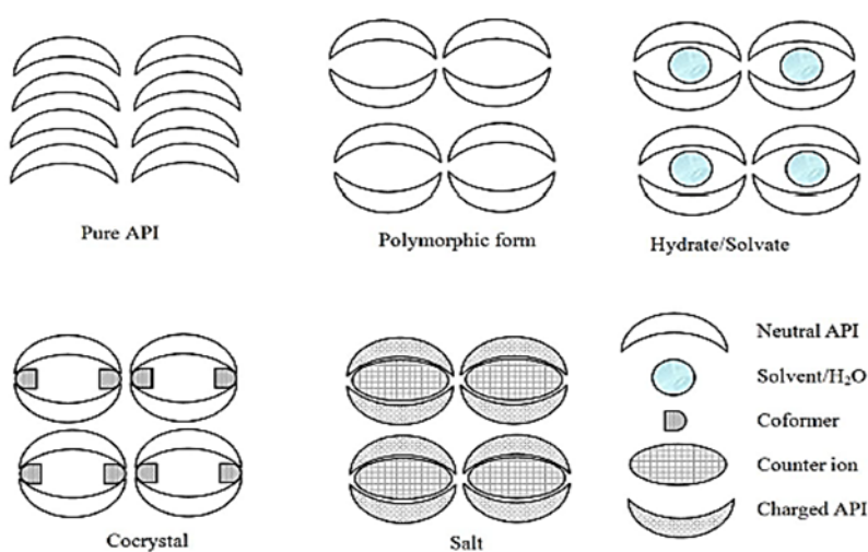
Figure 1: Schematics of salt, co-crystal, and polymorphism
