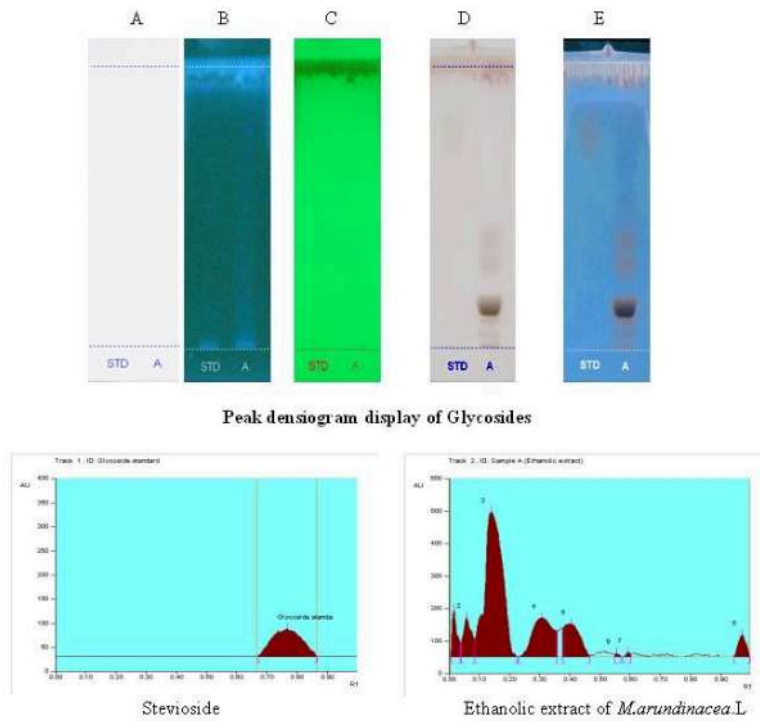
Fig. 5 Chromatograms of extract in HPTLC analysis for Glycosides. (A) Before derivatization under day light, (B) Under UV 366 nm (C) Under UV 254 nm, (D) After derivatization under day light, (E) Under UV 366 nm.
