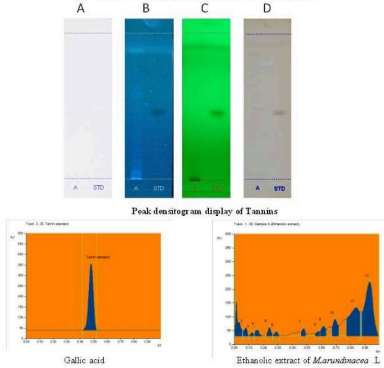
Fig. 4 Chromatograms of extract in HPTLC analysis for Tannins. (A) Before derivatization under day light, (B) Under UV 366 nm (C) Under UV 254 nm, (D) After derivatization under day light.
