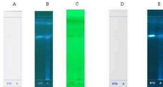
Fig. 1 Chromatograms of extract in HPILC analysis for Flavonoids. (A) Before derivatization under day light, (B) Under UV 366 nm (C) Under UV 254 nm, (D) After derivatization under day light, (E) Under UV 366nm.
