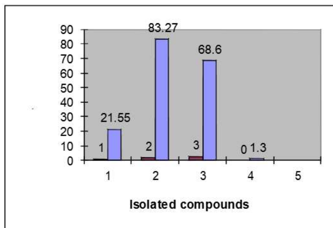
Figure 1: MICs in \mu M of isolated compounds against T. b. brucei
