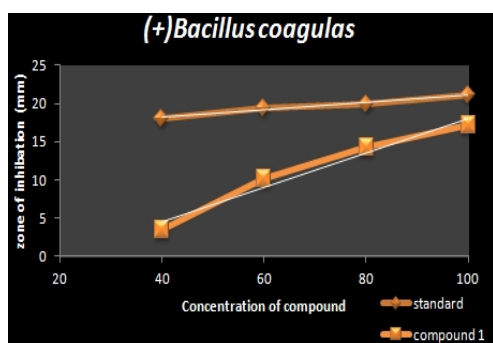
Fig 1. Screening activity of compound 1 with the spatial reference to streptomycin against Bacillus coagulans
