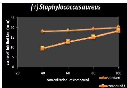
Fig 2 Screening activity of compound 1 with the spatial reference to streptomycin against Staphylococcus aureus
