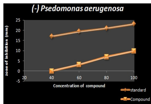
Fig 4. Screening activity of compound 1 with the spatial reference to streptomycin against Pseudomonas aeruginosa
