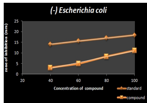
Fig 3. Screening activity of compound 1 with the spatial reference to and streptomycin against Escherichia coli .
