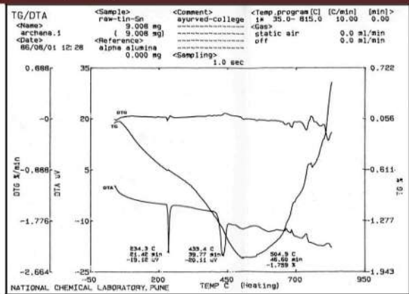
Figure 5: TG/DTA Analysis of Raw Vanga
