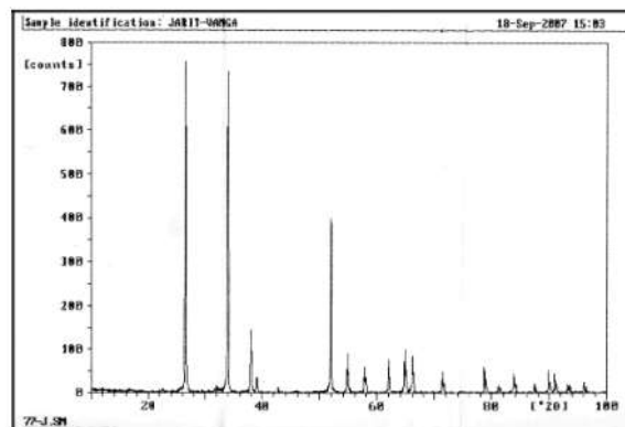
Figure 3: XRD Analysis of Jarit Vanga
