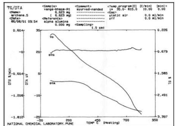
Figure 7: TG/DTA Analysis of Vanga Bhasma
