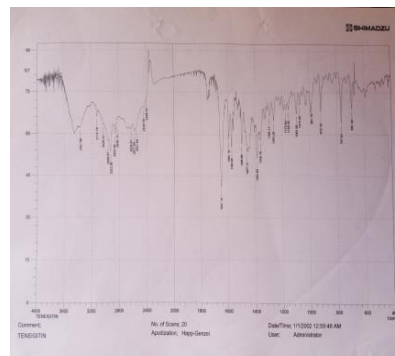
Fig 8: Infrared Spectrum of Pure Teneligliptin drug
