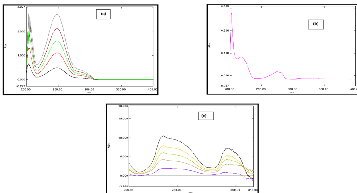
Figure 4: Spectra of PCM (a) divided by spectra of 4 \mu\text{g mL}^{-1} TAP (b) Derivative Ratio spectra (c)
