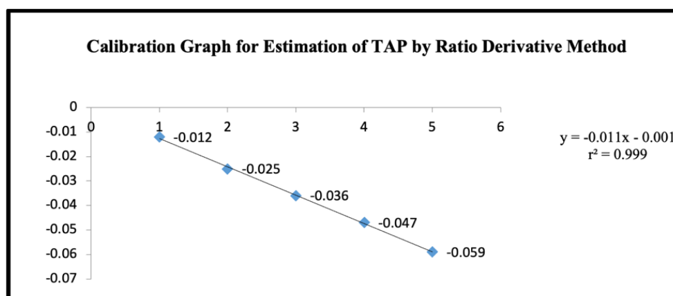
Figure 1: Calibration Graph for Estimation of TAP Using 13 \mu\text{g mL}^{-1} of PCM as Divisor Concentration
