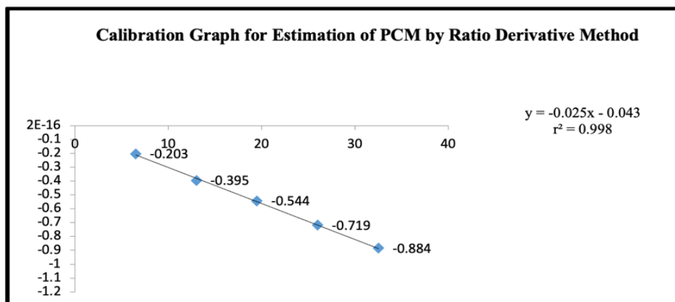
Figure 2: Calibration Graph for Estimation of PCM Using 4 \mu\text{g mL}^{-1} of TAP as Divisor Concentration
