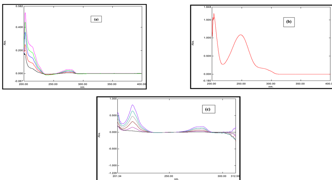
Figure 3: Spectra of TAP (a) divided by spectra of 13 \mu\text{g mL}^{-1} PCM (b) Derivative Ratio spectra (c)
