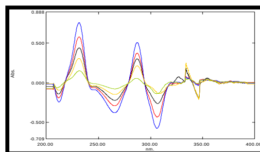
Figure 6: Ratio Derivative Spectra of PCM (6.5, 13, 19.5, 26, and 32.5 \mu\text{g mL}^{-1} )
