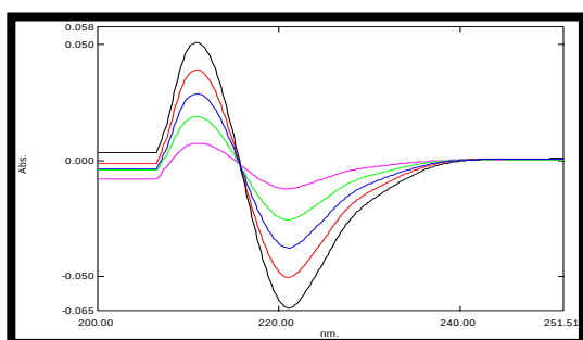
Figure 5: Ratio Derivative Spectra of TAP (1, 2, 3, 4, and 5 \mu\text{g mL}^{-1} )
