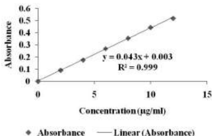
Figure 1: Calibration curve of Ibuprofen in pH 7.2 phosphate buffer ( \lambda_{max} = 221 \text{ nm} )
