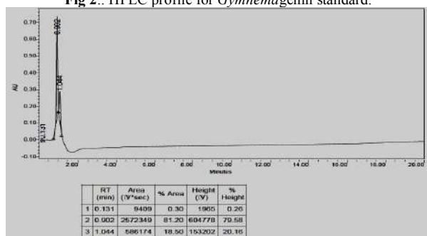
Fig 2: HPLC profile for Gymnemenin standard.
