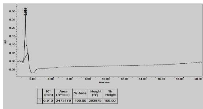
Fig 4: HPLC profile for control
