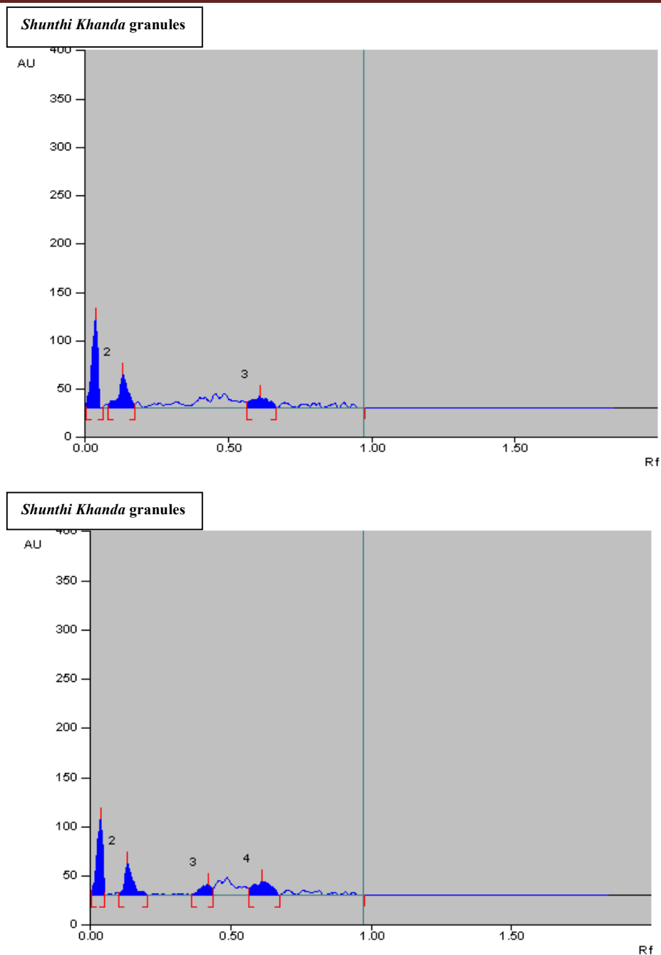
Figure No.1 Densitogram curve of Shunthi Khanda Granules Extract in 254nm & 366nm
