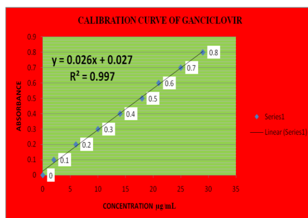
Figure 3: Calibration Curve of Ganciclovir
