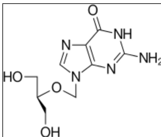
Figure 1: Molecular Structure of Ganciclovir
