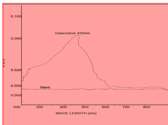
Figure 2: UV Visible Spectrum of Ganciclovir
