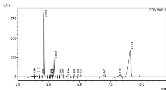
Figure 1: Chromatogram of ABZ and its degradation products - albendazole sulfoxide (ricobendazole) and albendazole sulfone at a concentration of 100 \mu\text{g mL}^{-1}
