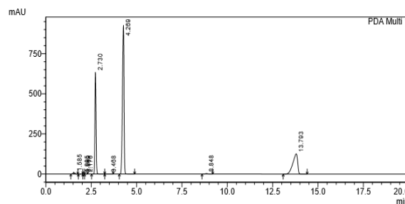
Figure 2: Chromatogram of FBZ and its degradation products - fenbendazole sulfoxide (oxfendazole) and fenbendazole sulfone at a concentration of 100 \mu\text{g mL}^{-1}
