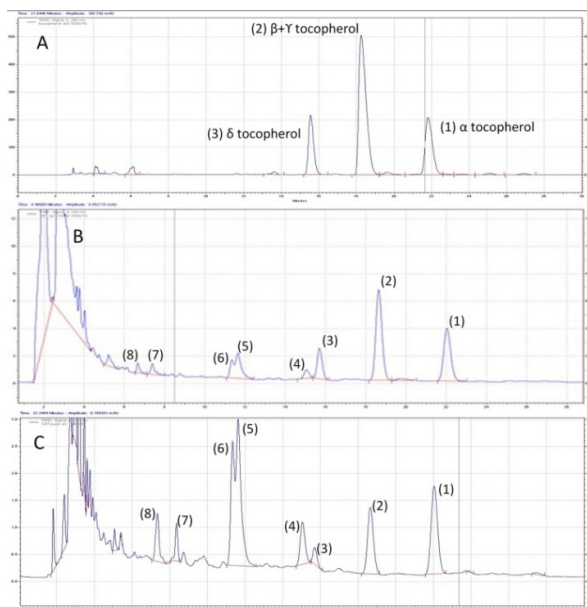
Figure 3: Chromatograms of the tocopherols: Standard (A), SCF (B) and Solvent (C) extractions. Peaks: 1: \alpha -tocopherol, 2: \beta + \gamma -tocopherol, 3: \delta -tocopherol, 4: unidentified, 5,6,7,8: tocotrienols
