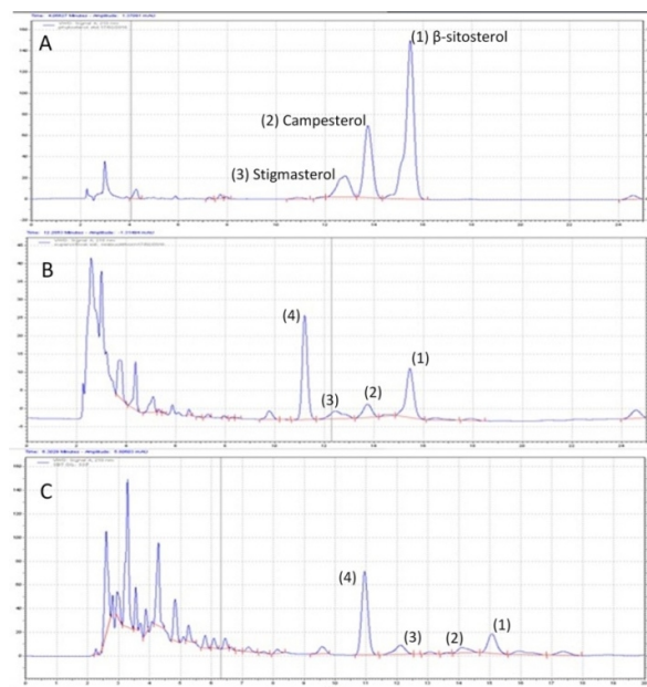
Figure 4: Chromatograms of the phytosterols: Standard (A), SCF (B) and Solvent (C) extractions. Peaks: 1: \beta -sitosterol, 2: Campesterol 3: Stigmasterol, 4: unidentified
