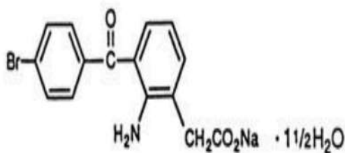
Figure 1: Structure of bromfenac sodium 4
