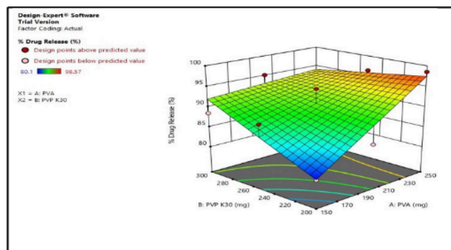
Figure 3: Surface response plot showing effect of polyvinyl alcohol and polyvinyl pyrrolidone K-30 on drug release
