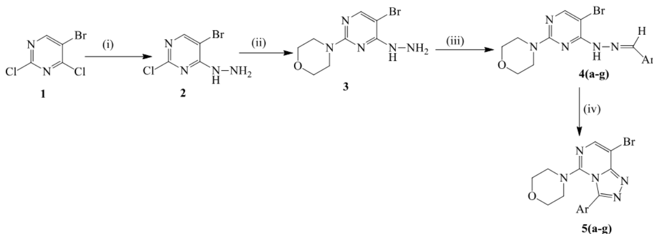
Scheme 1: Synthetic pathway for the 1,2,4-triazole derivatives ( 5a-g )
