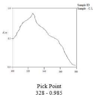
Figure 1: UV of Citrus limonum peel ethanol extract
