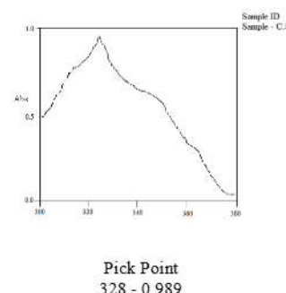
Figure 2: UV of Citrus sinensis peel ethanol extract
