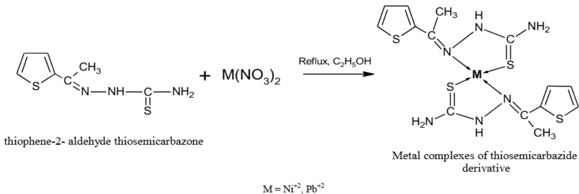
Figure 3: Synthesis of metal complexes [M(L) 2 ]Cl 2
