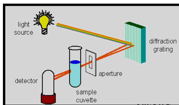
Figure 1: UV Visible single beam Spectrophotometer.
