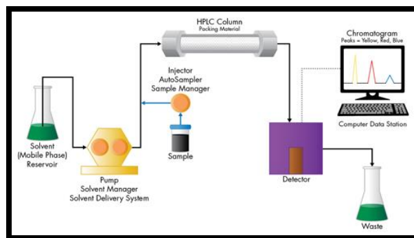
Figure 4: Isocratic HPLC system
