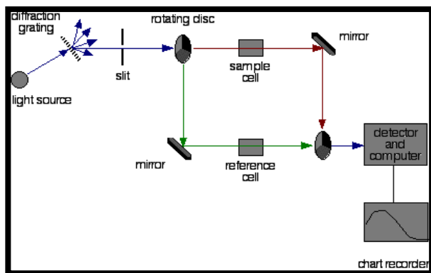
Figure 2: UV Visible double beam Spectrophotometer.
