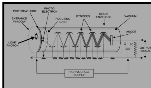
Figure 3: Photo Multiplier Tube.
