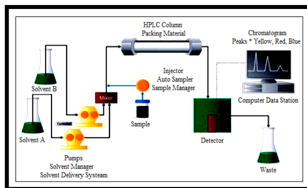
Figure 5: High Pressure Gradient HPLC System
