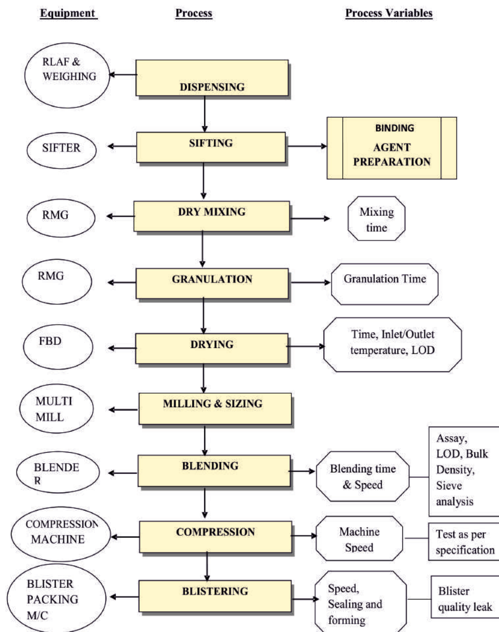
Process Flow Diagram
